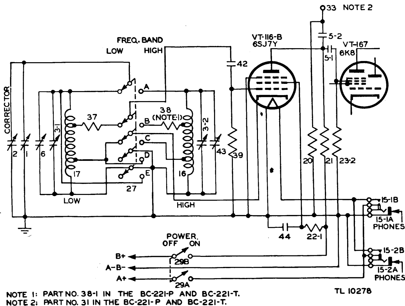
Figure 75. Frequency Meters BC-221-P, BC-221-T, and BC-221-AF, functional diagram, variable frequency oscillator circuit.
