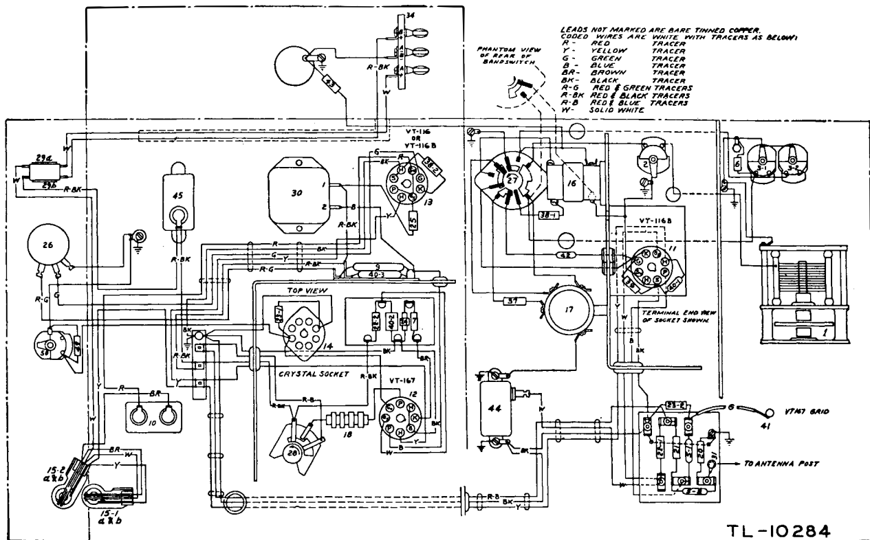
Figure 81. Frequency Meters BC-221-P and BC-221-T, chassis wiring diagram.
