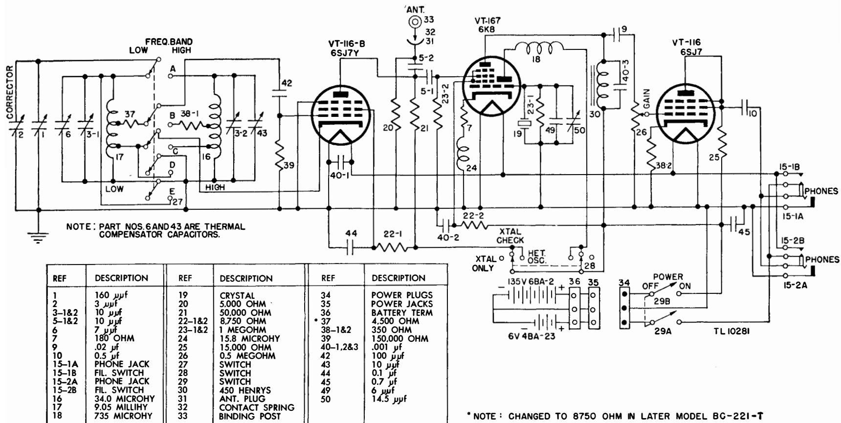
Figure 78. Frequency Meters BC-221-P and BC-221-T, schematic diagram.
