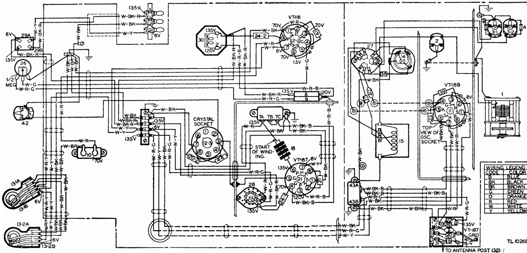
Figure 65. Frequency Meters BC-221-O and BC-221-R, chassis wiring diagram.
