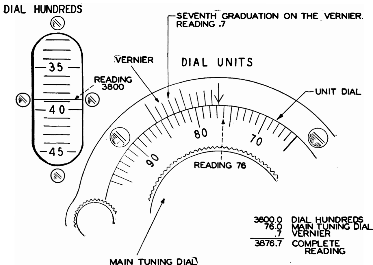
Figure 13. Frequency Meter BC-221-(&CircledS), main tuning dial.
