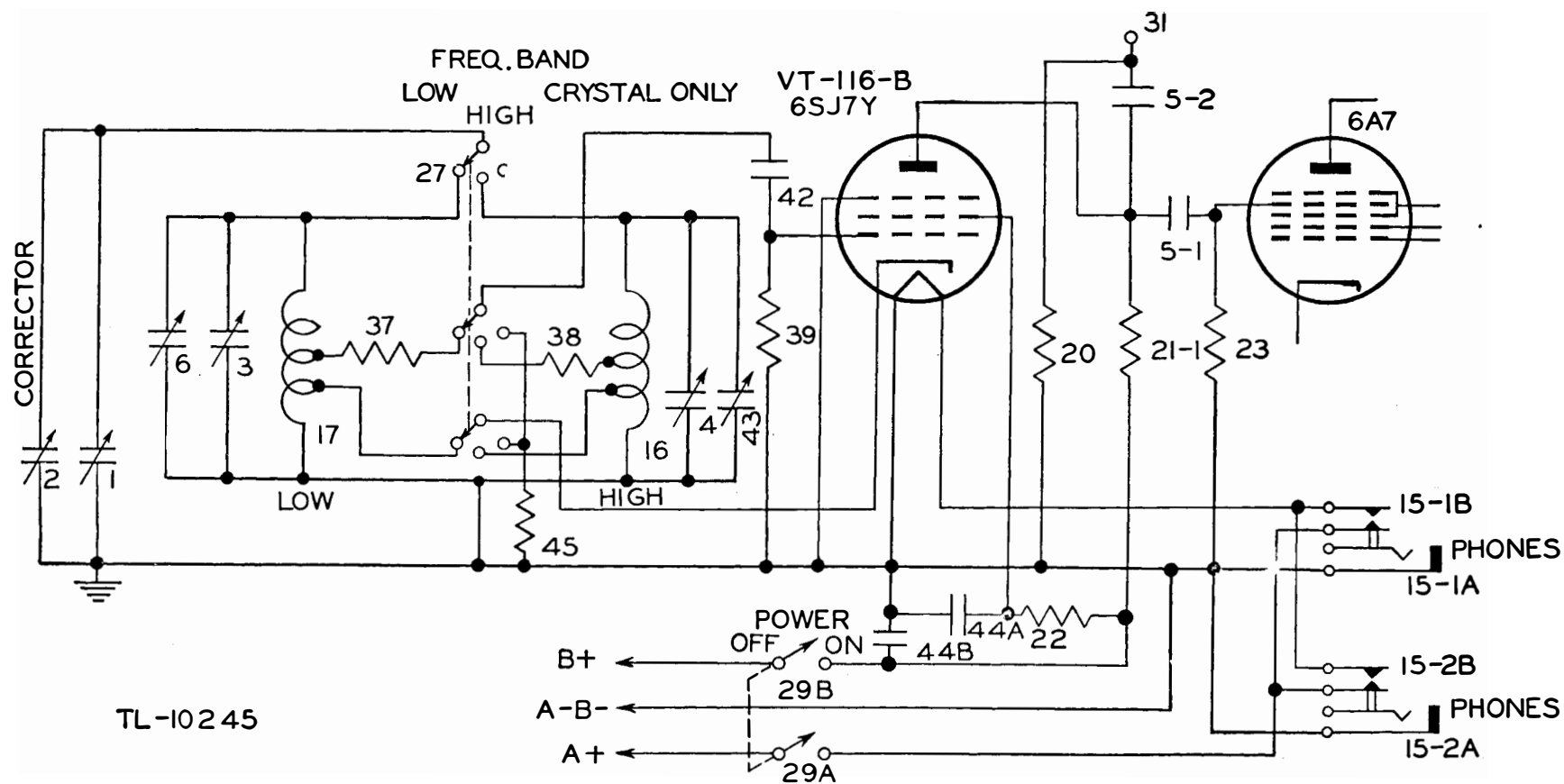
Figure 52. Frequency Meter BC-221-(3), functional diagram, variable frequency oscillator circuit.
