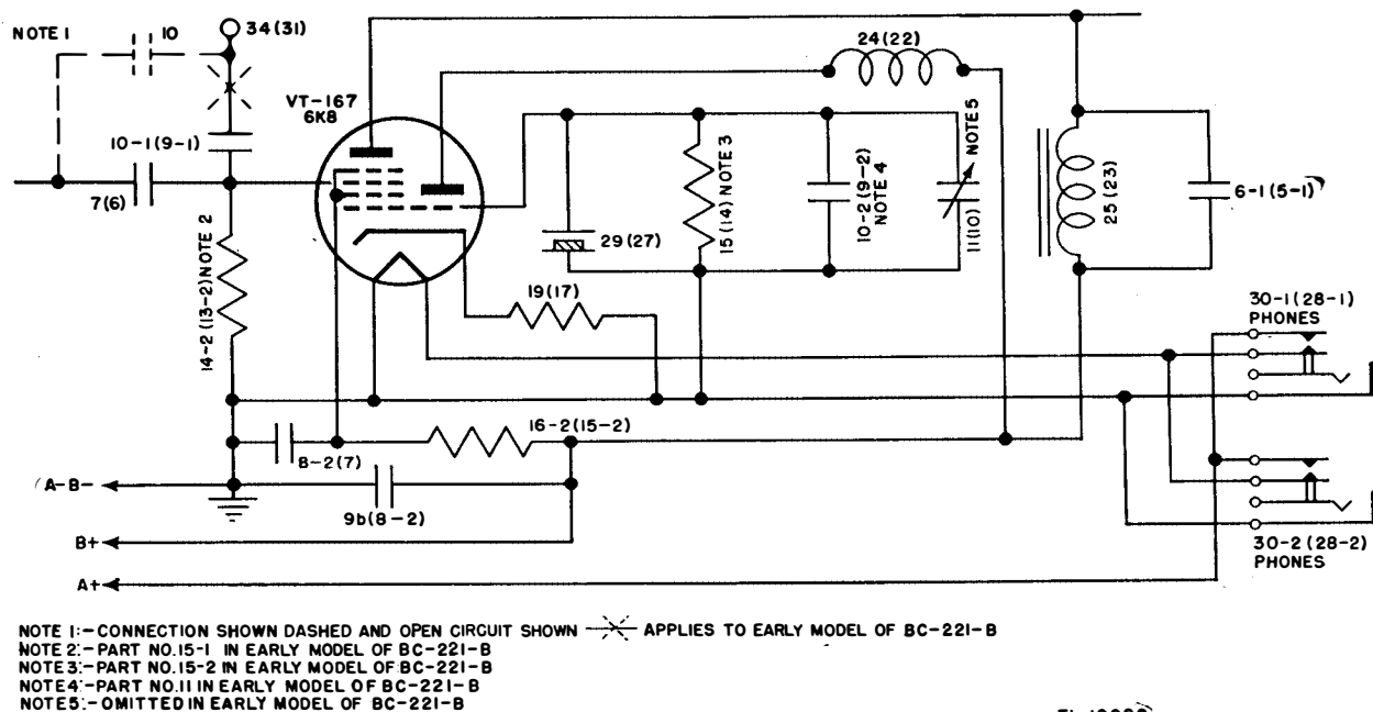
Figure 37 Frequency Meter BC-221-(2), functional diagram, crystal-oscillator circuit.
