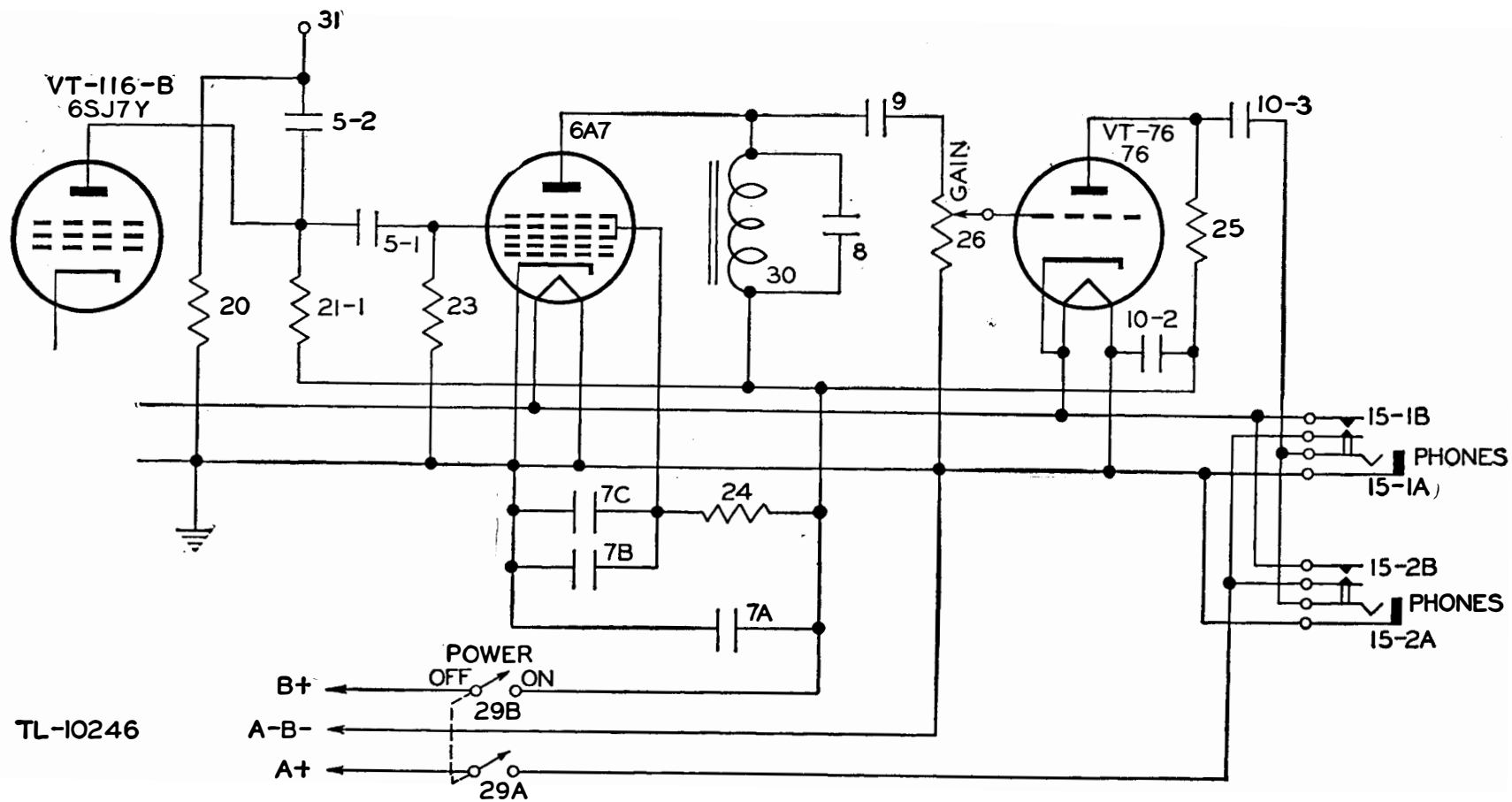
Figure 53. Frequency Meter BC-221-(3), functional diagram, detector and audio-amplifier circuits.
