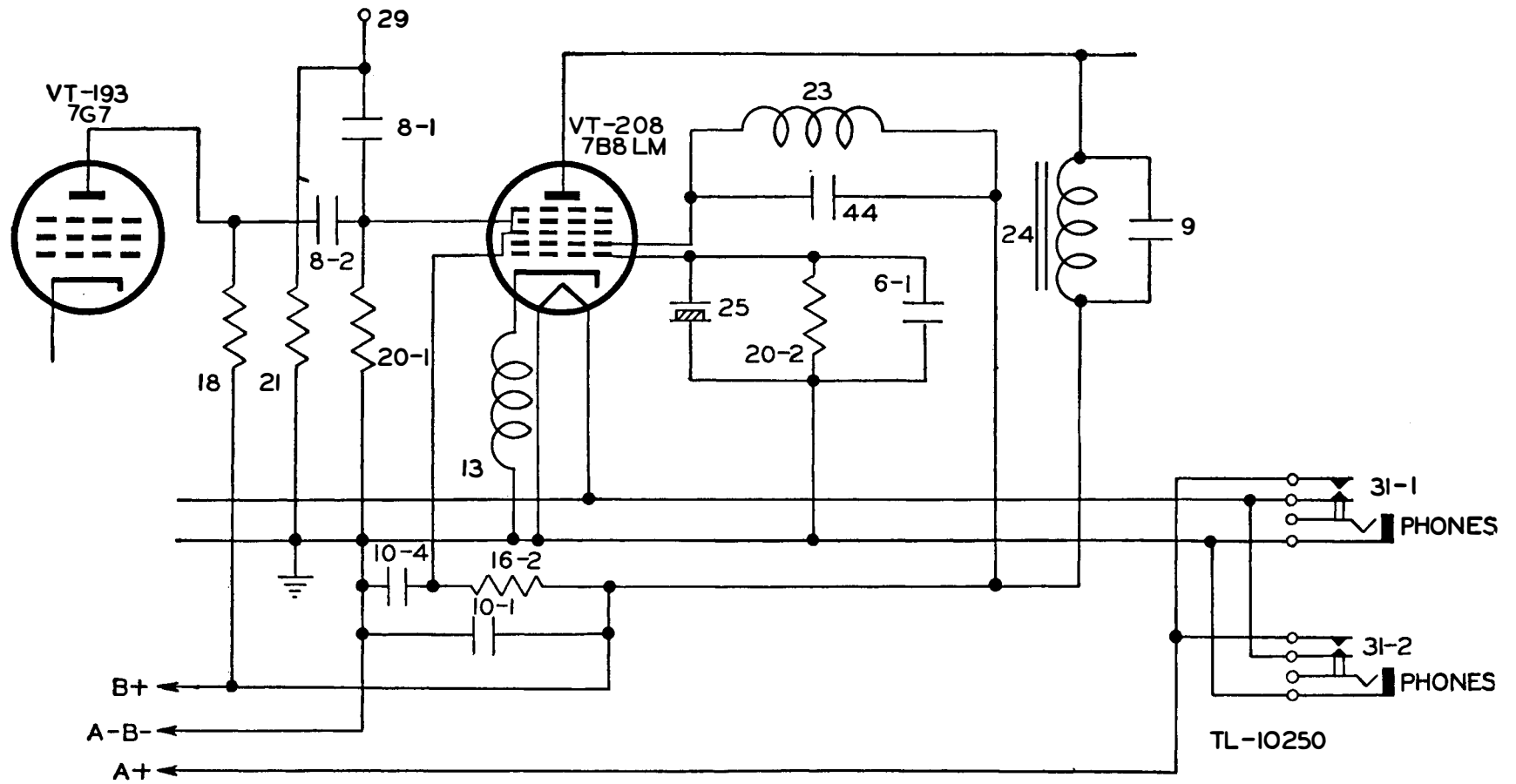
Figure 46. Frequency Meter BC-221-E, functional diagram, crystal-oscillator circuit.
