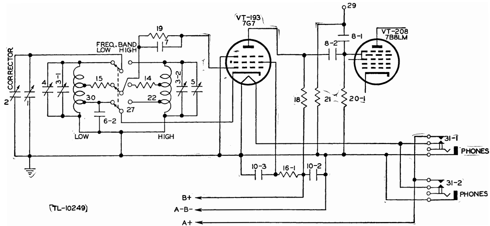
Figure 47. Frequency Meter BC-221-E, functional diagram, variable frequency oscillator circuit.
