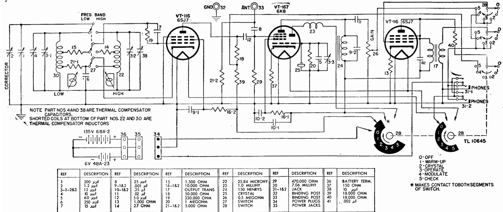
Figure 94. Frequency Meter BC-221-AK, schematic diagram.
