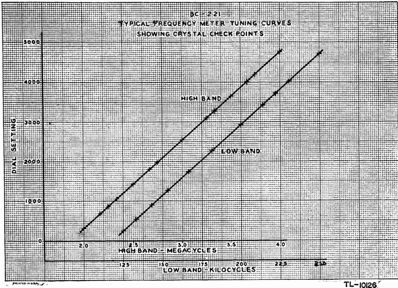
Figure 16. Frequency Meter BC-221-( \& ), typical frequency meter tuning curves.
