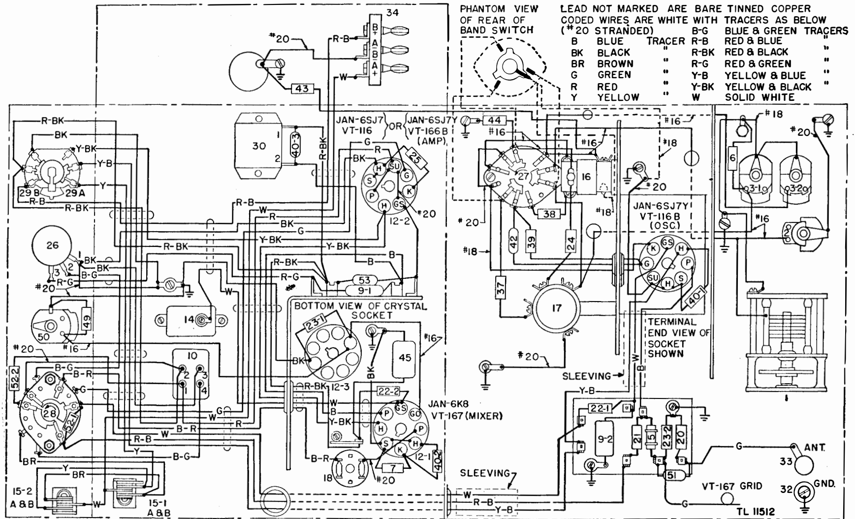
Figure 102. Frequency Meter BC-221-AL, chassis wiring diagram.
