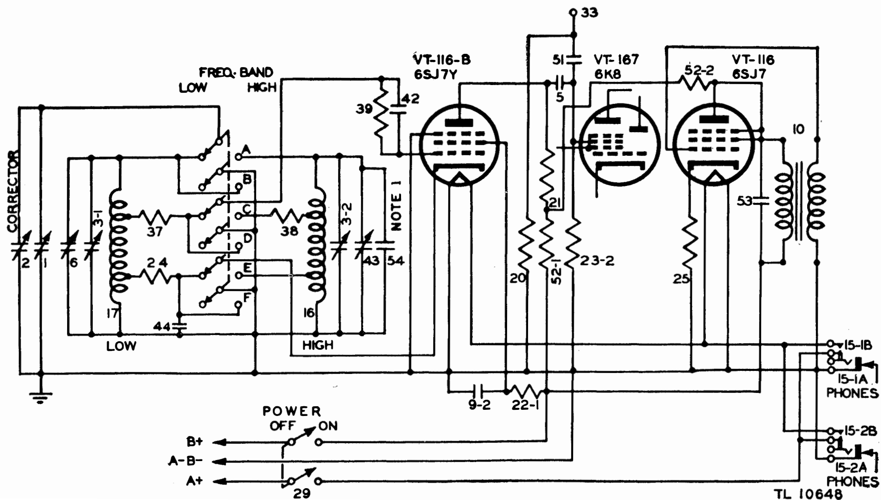
Figure 97. Frequency Meter BC-221-(8), functional diagram, variable frequency oscillator and audio-modulator circuits.
