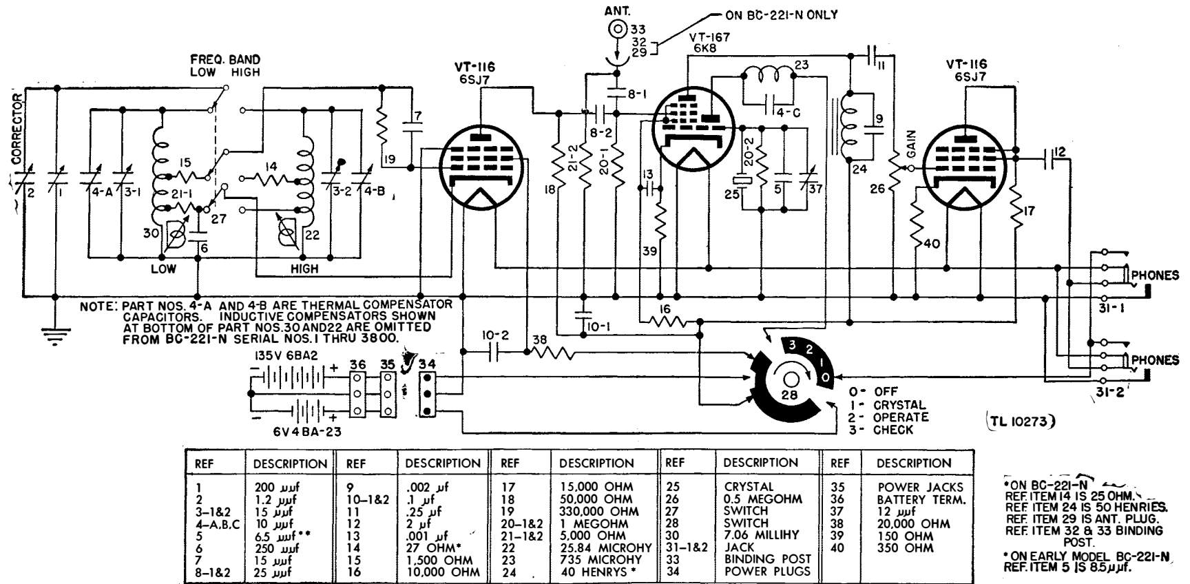
Figure 71. Frequency Meters BC-221-N and BC-221-AA, schematic diagram.
