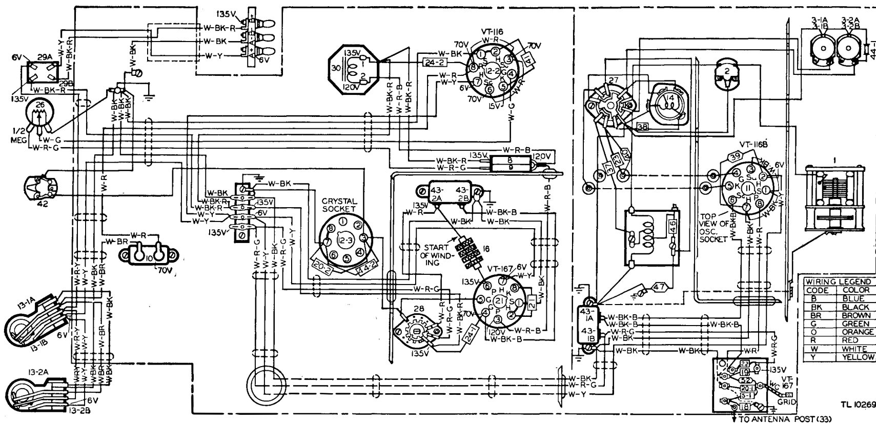
Figure 66. Frequency Meter BC-221-AC, chassis wiring diagram.
