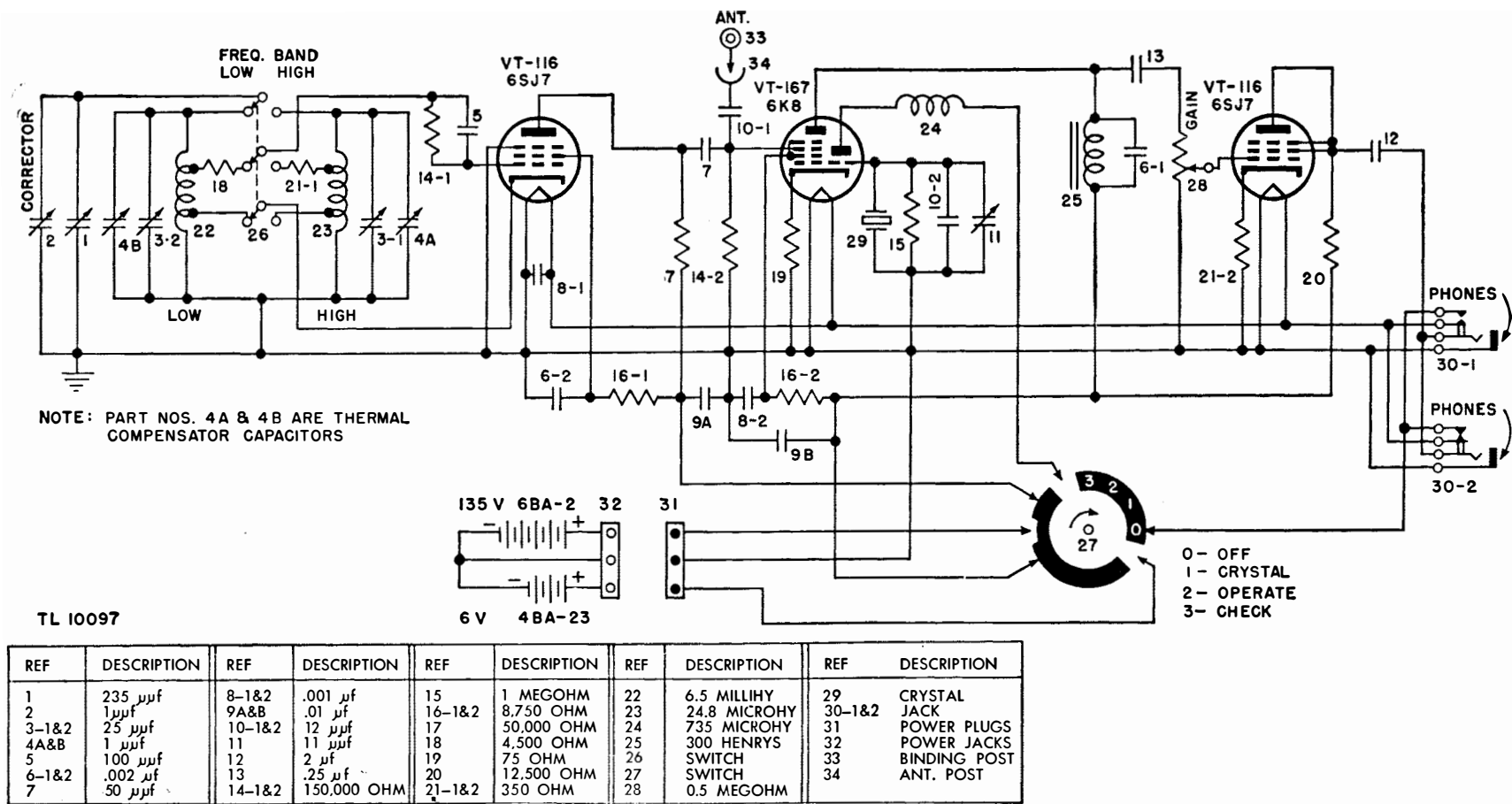
Figure 41. Frequency Meter BC-221-B (late model), schematic diagram.
