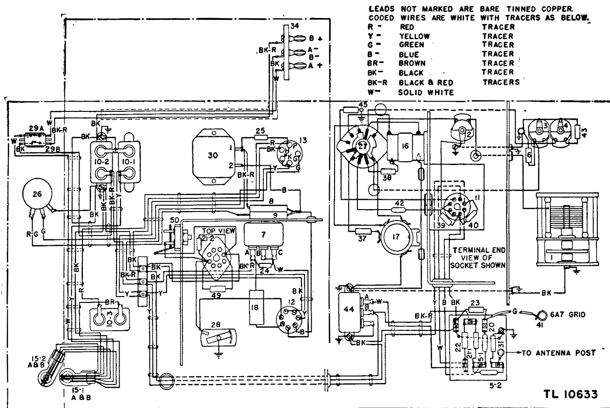
Figure 55. Frequency Meter BC-221-(3), chassis wiring diagram.
