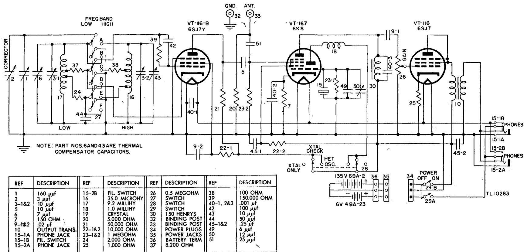
Figure 80. Frequency Meter BC-221-AH, schematic diagram.
