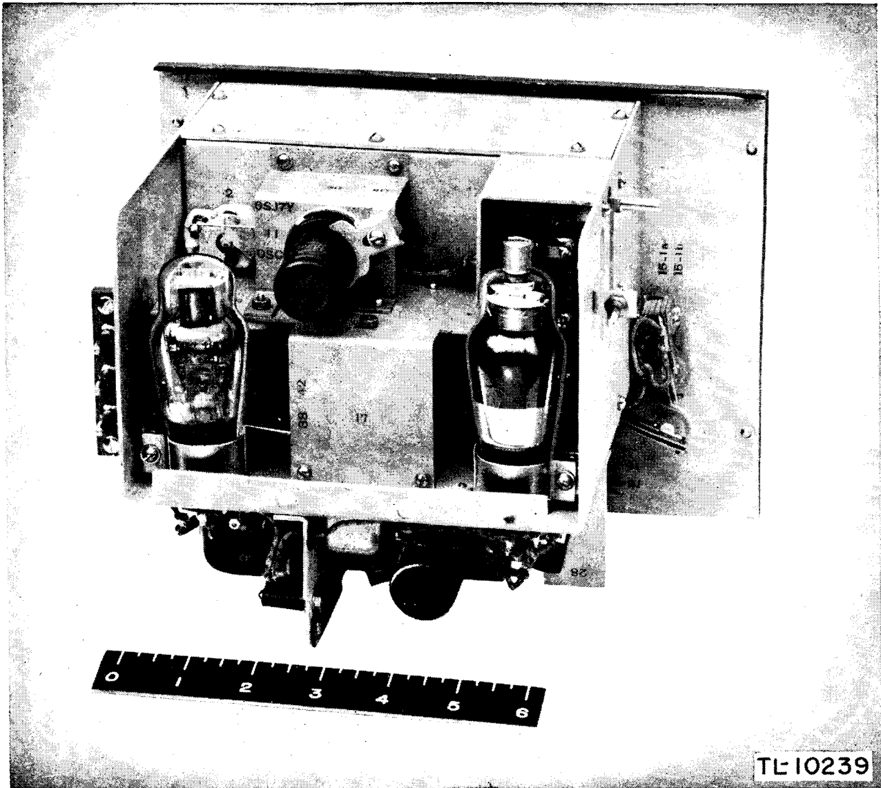
Figure 22. Frequency Meter BG-221-F, rear view of chassis.
