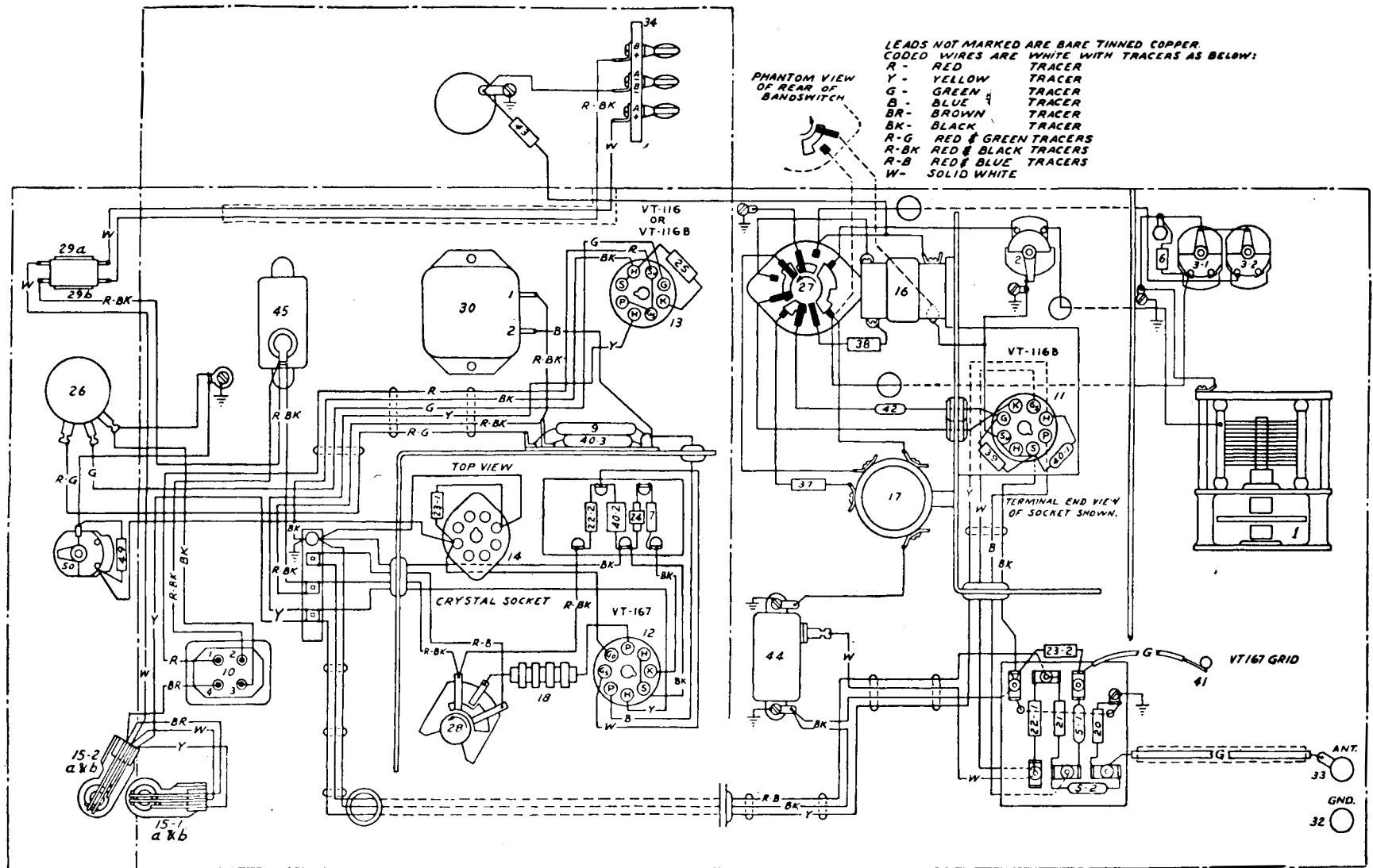
Figure 82. Frequency Meter BC-221-AF, chassis wiring diagram.
