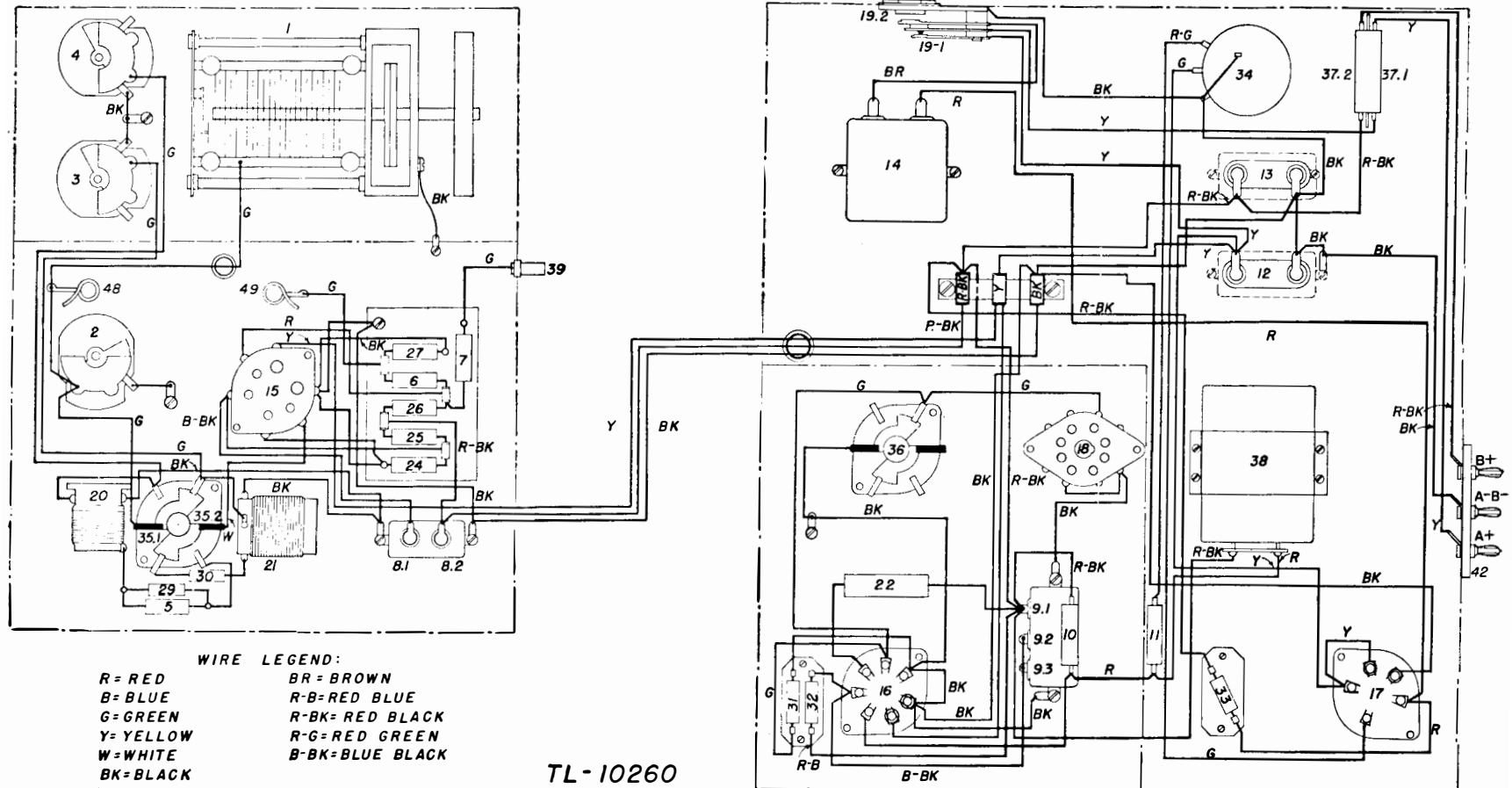
Figure 33. Frequency Meter BC-221-A, chassis wiring diagram.
