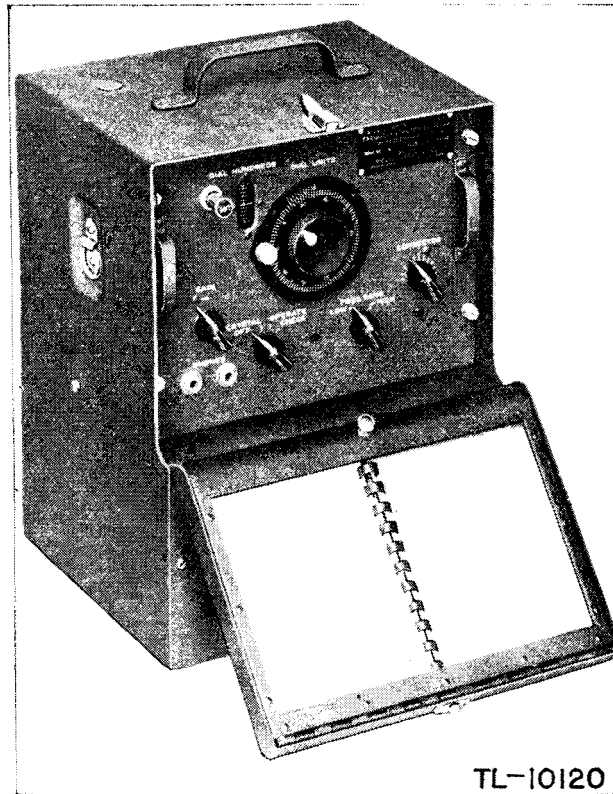
Figure 1. Frequency Meter BC-221-(G), in metal cabinet.
