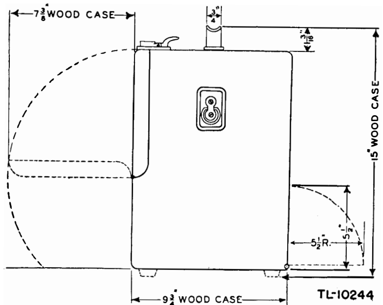
Figure 27. Frequency Meter BC-221-(G), typical dimensions, wooden cabinet (subject to slight variations).
