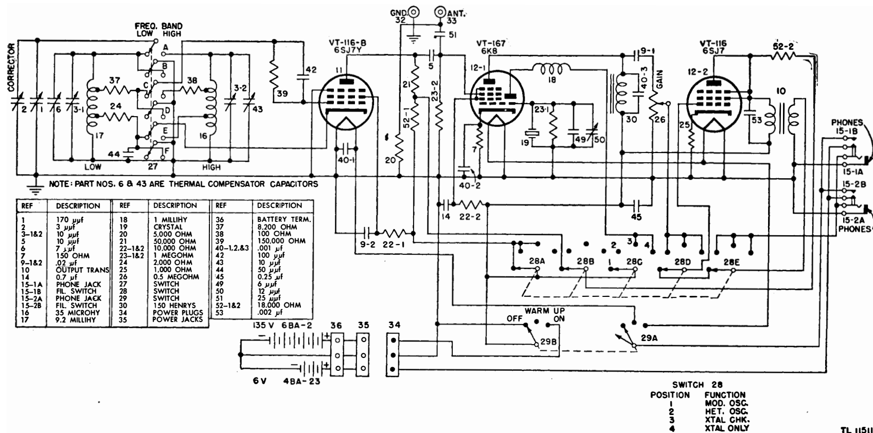
Figure 100. Frequency Meter BC-221-AL, schematic diagram.
