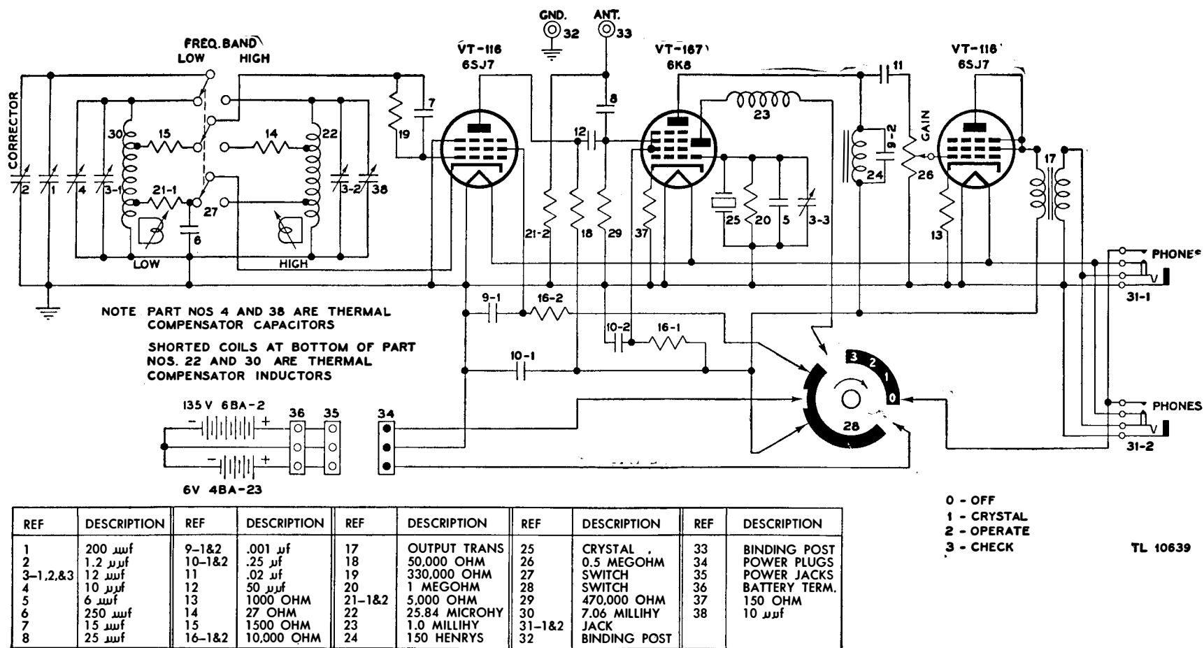
Figure 88. Frequency Meter BC-221-AG, schematic diagram.
