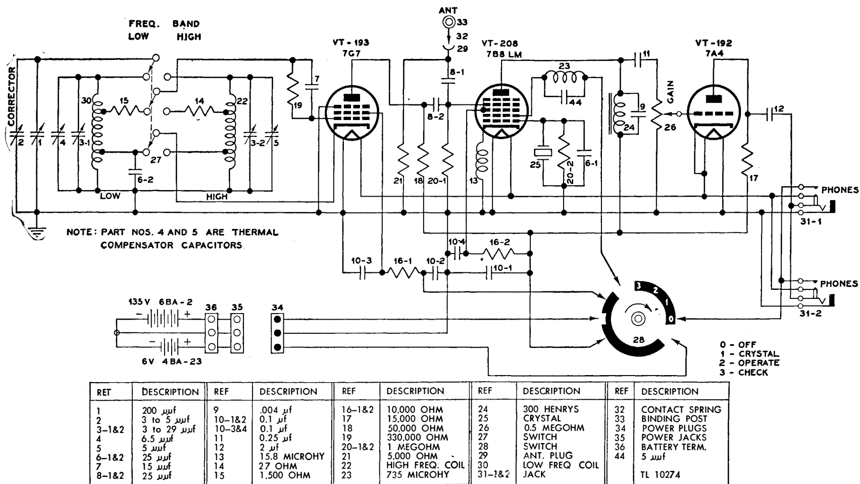
Figure 49. Frequency Meter BC-221-E, schematic diagram.
