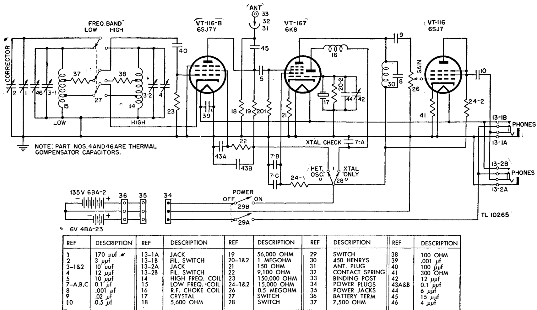
Figure 62. Frequency Meters BC-221-O and BC-221-R, schematic diagram.
