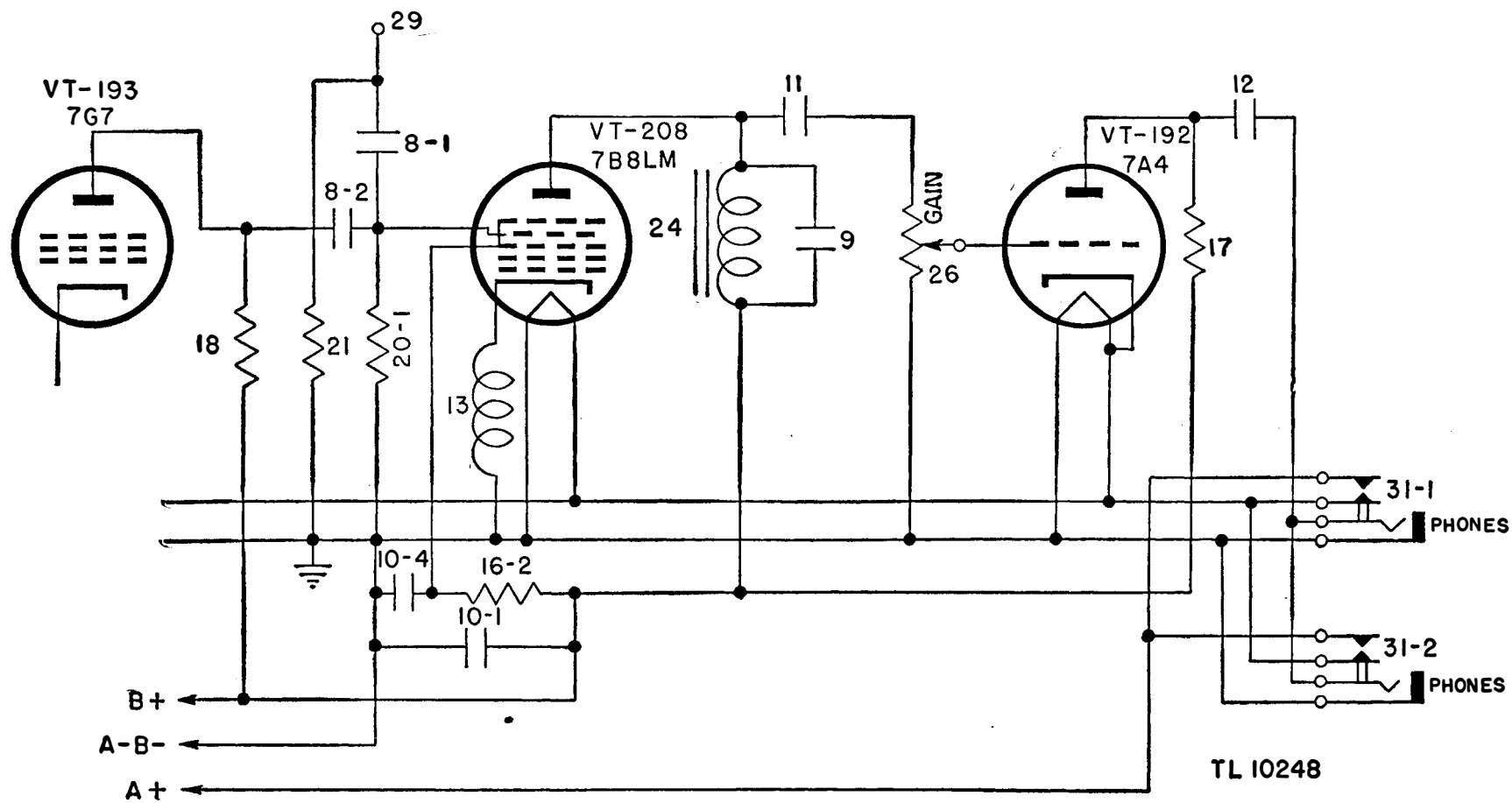
Figure 48. Frequency Meter BC-221-E, functional diagram, detector and audio-amplifier circuits.
