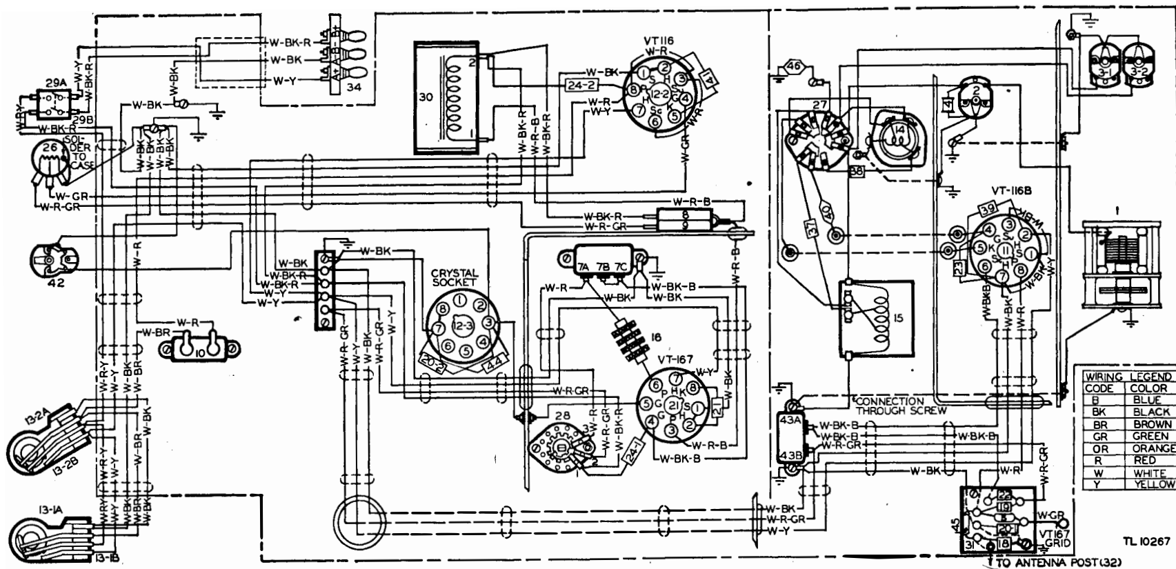
*Figure 64. Frequency Meter BC-221-M, chassis wiring diagram.
