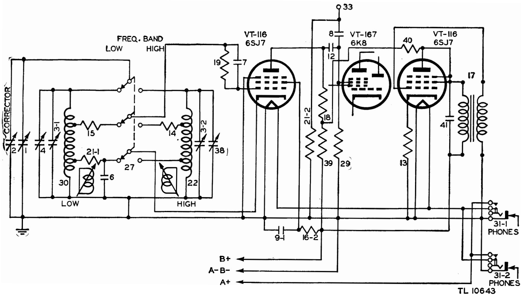
Figure 92. Frequency Meter BC-221-AK, functional diagram, variable frequency oscillator and audio-modulator circuits.
