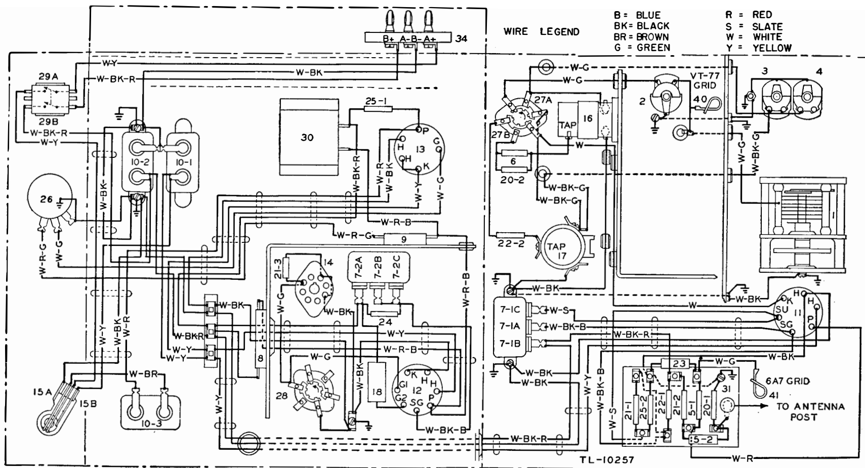
Figure 34. Frequency Meters BC-221-C and BC-221-D, chassis wiring diagram.
