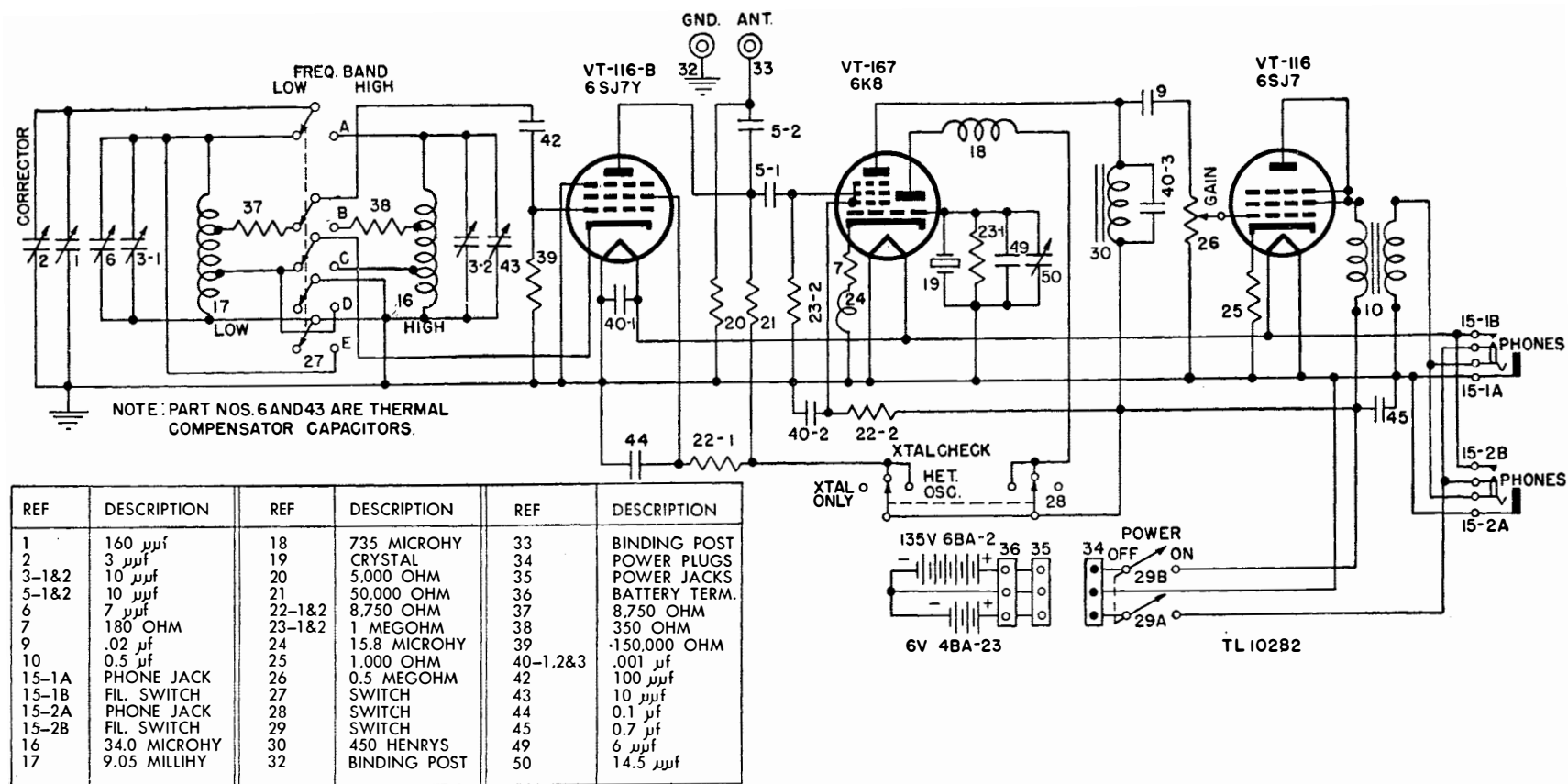
Figure 79. Frequency Meter BC-221-AF, schematic diagram.
