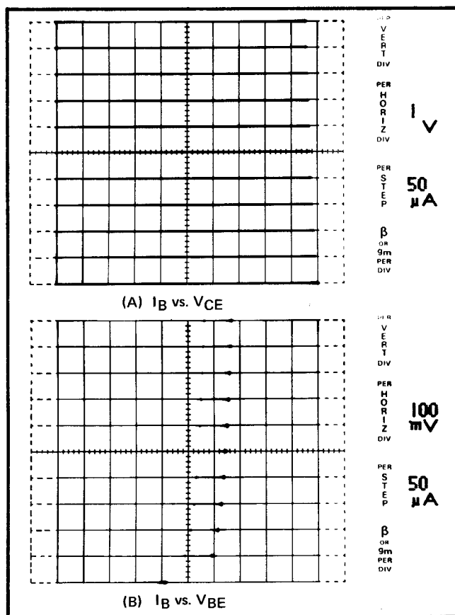
Fig. 2-14. (A) I_B vs. V_{CE} , I_b @ 50 \mu\text{A} per division; (B) I_B vs. V_{BE} , I_b @ 50 \mu\text{A} per division.
