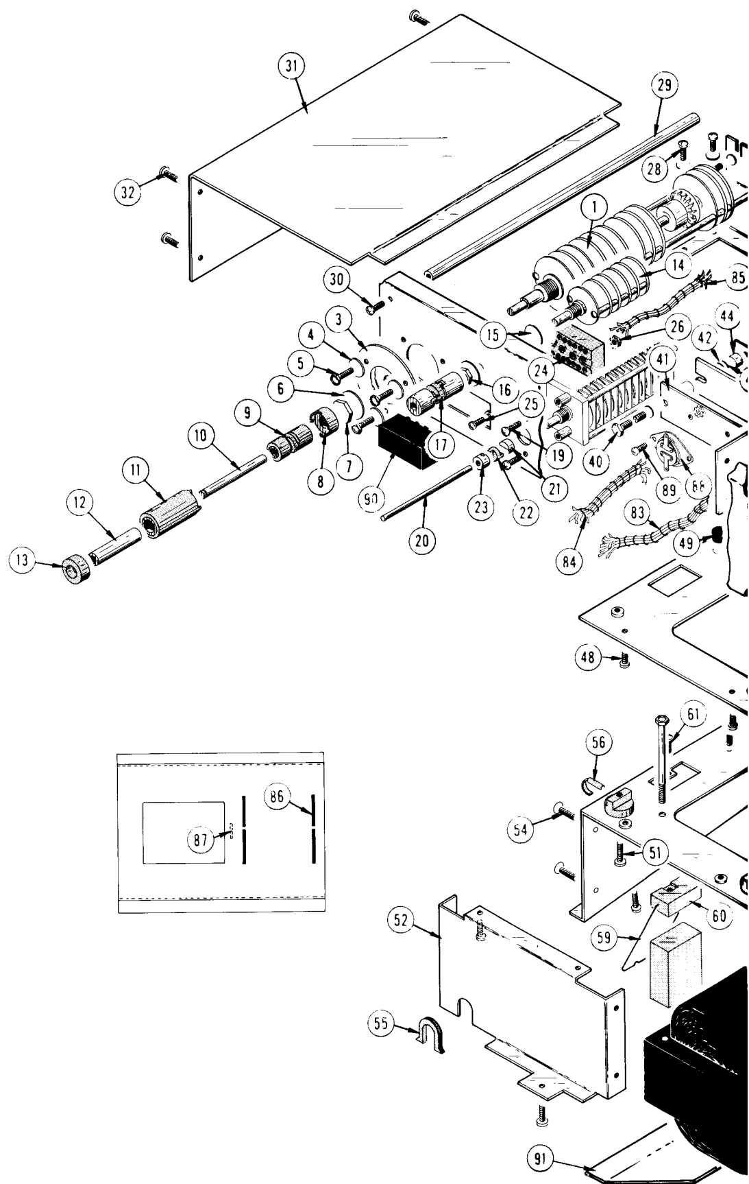
FIG. 4 COLLECTOR SUPP
