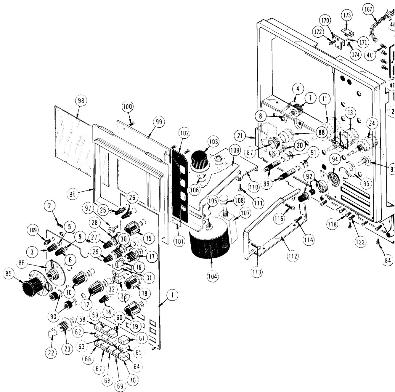
FIG. 1 FRONT
