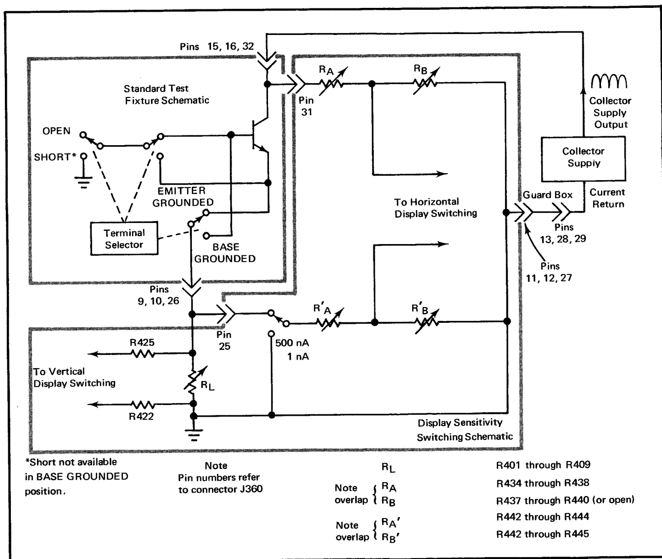
Fig. 3-10. Simplified schematic of Display Sensitivity switching and Standard Test Fixture schematics for measurement of emitter current ( I_E ), collector-base current ( I_{CBO} ), collector-emitter voltage ( V_{CE} ) or collector-base voltage ( V_{CB} ).
