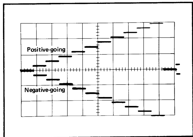
Fig. 2-24. Step Generator output in both polarities
