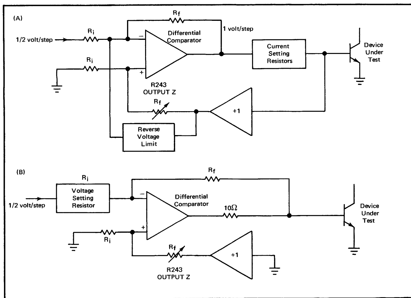
Fig. 3-7. Block diagram of Step Output Amplifier: (A) Current Mode, (B) Voltage Mode.
