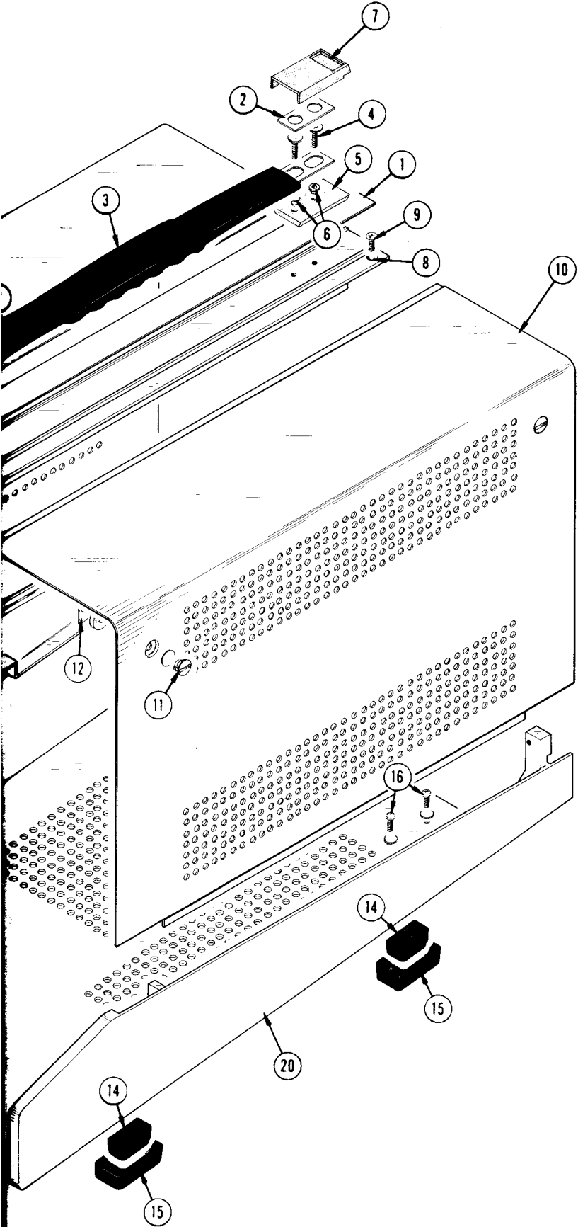
FIG. 6 CABINET
