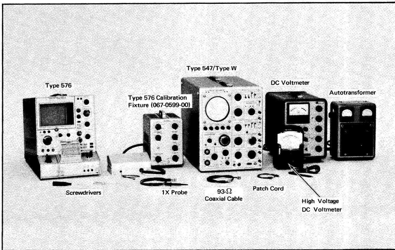
Fig. 5-1. Type 576 and test equipment.
