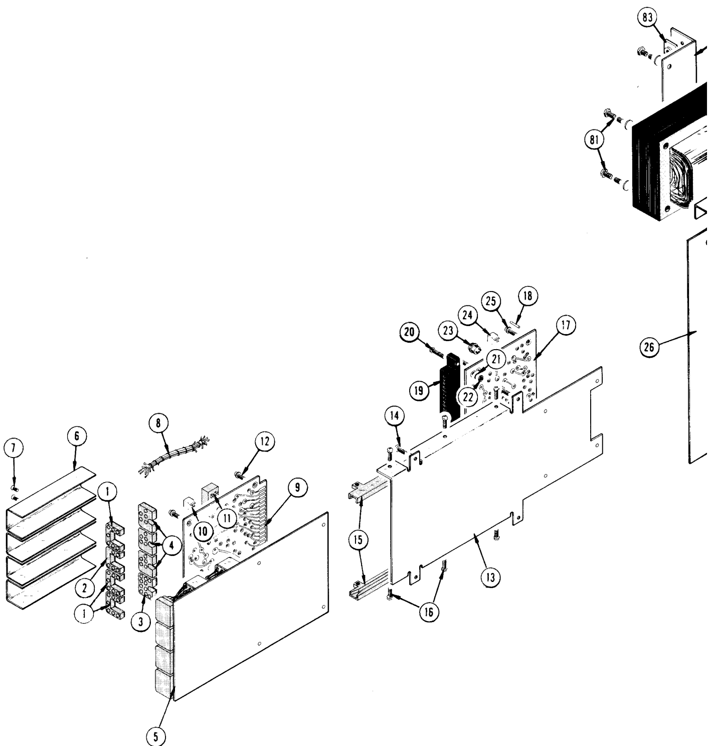
FIG. 3 CHASSIS
