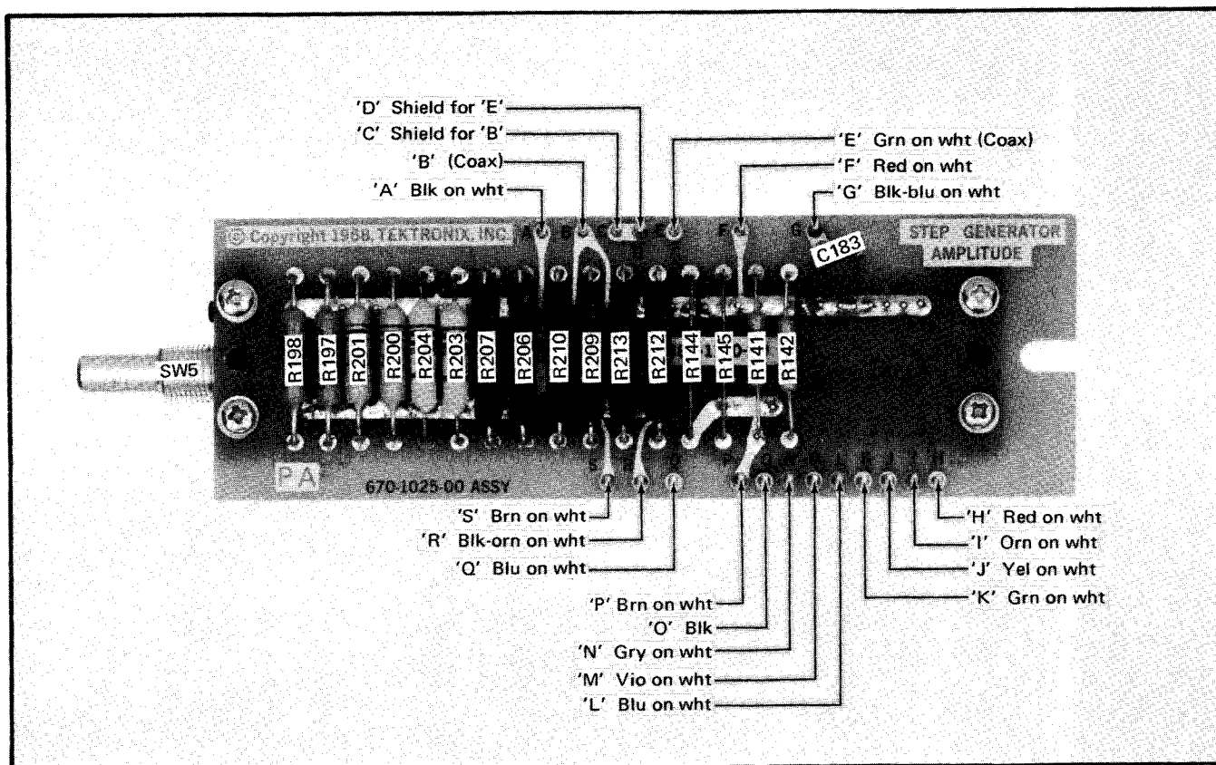
Fig. 4-8. Component locations and wiring color codes on Step Generator Amplitude circuit board.
