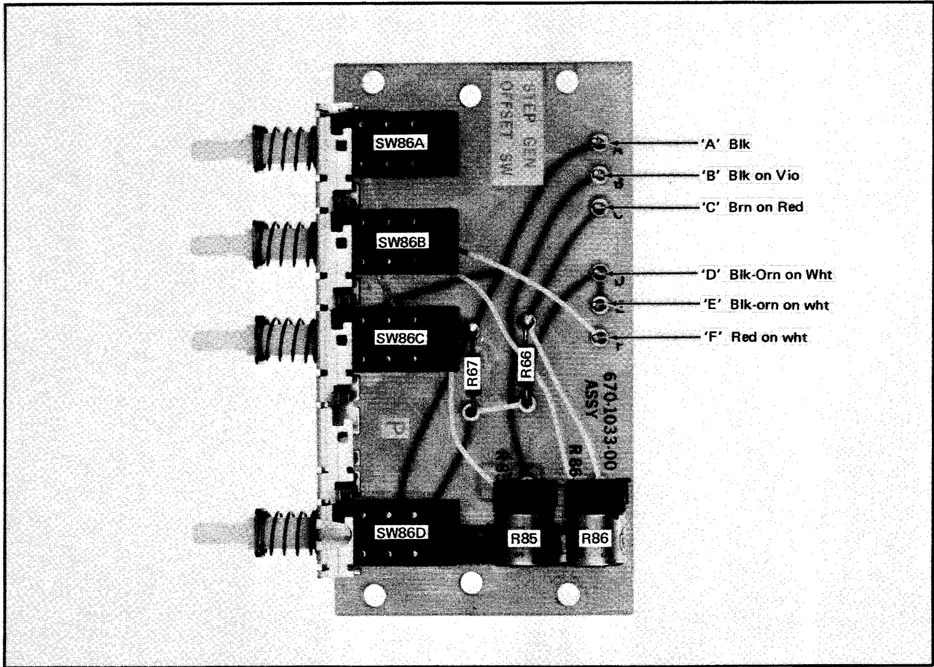
Fig. 4-9. Component locations and wiring color codes on Step Gen Offset circuit board.
