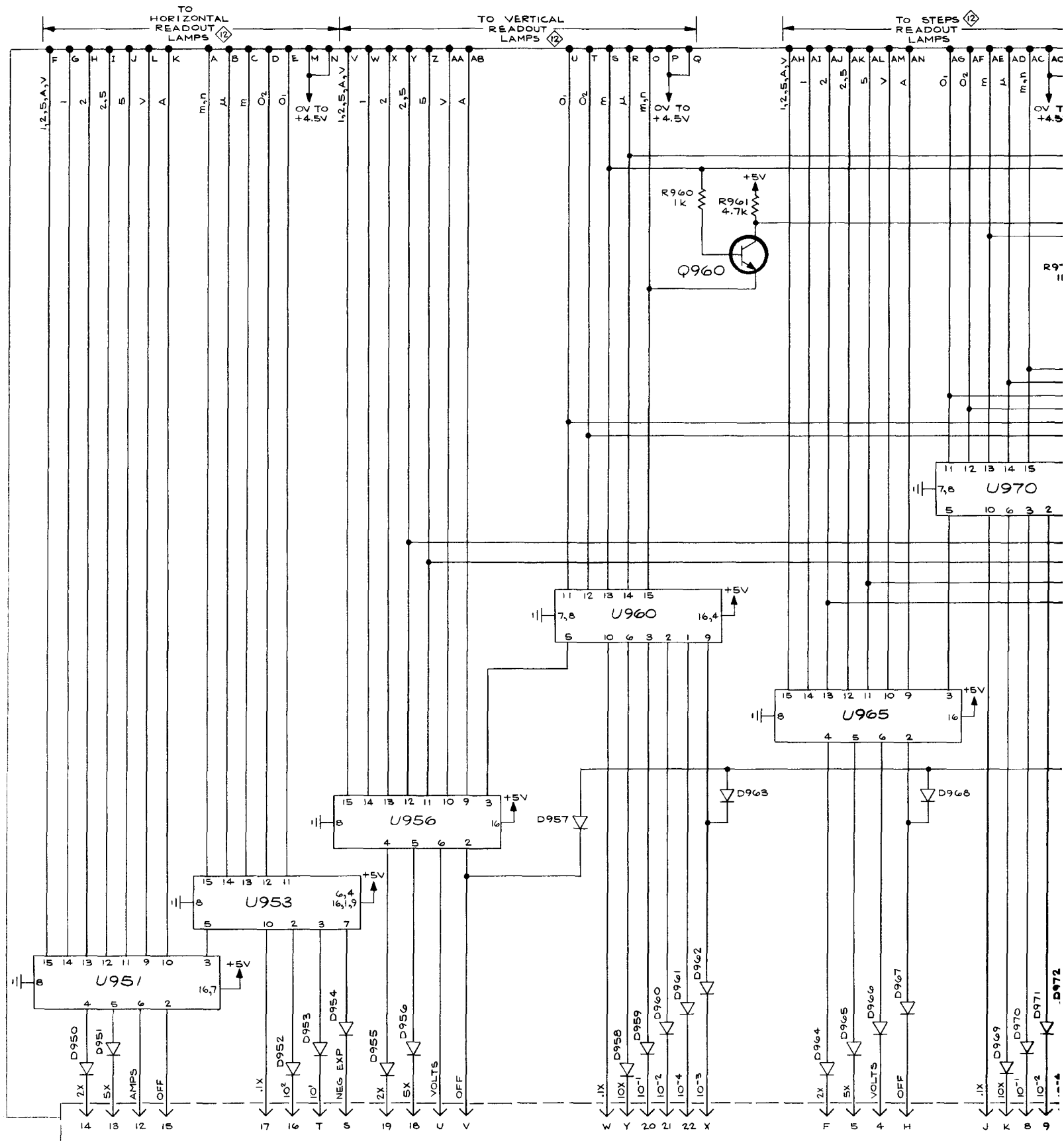
REFERENCE DIAGRAM 12 READOUT LAMPS
