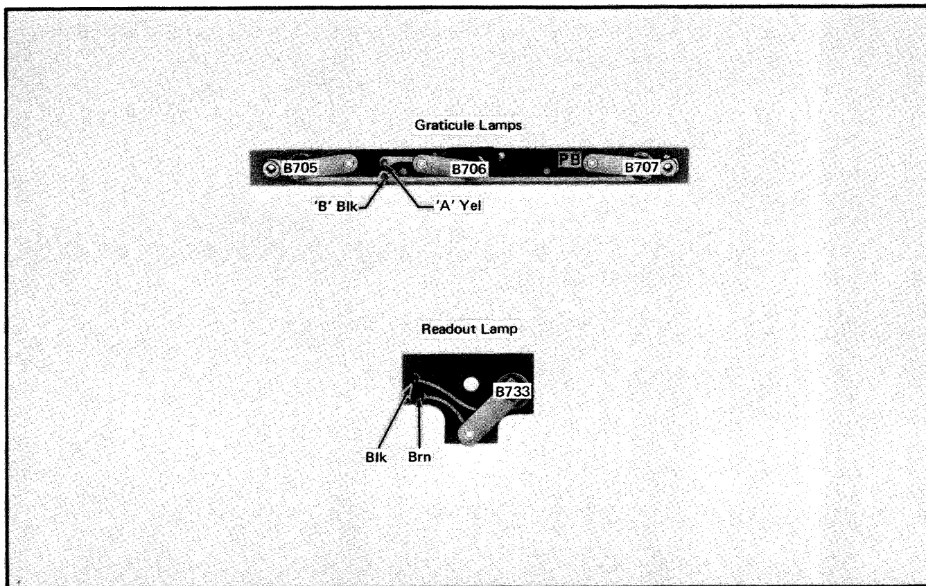
Fig. 4-25. Component locations and wiring color codes for Grat. Lamps and Readout Lamp circuit boards.
