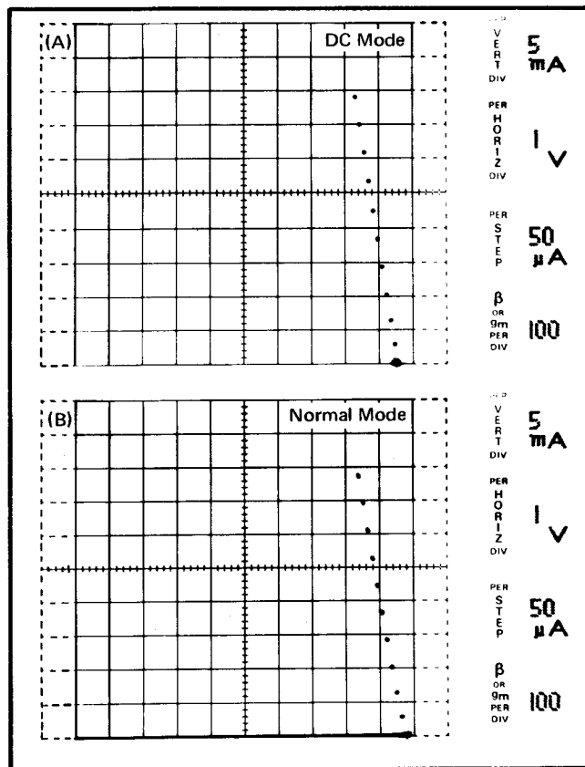
Fig. 2-16. 300 \mu\text{s} PULSED STEPS, (A) DC mode; (B) Normal mode.
