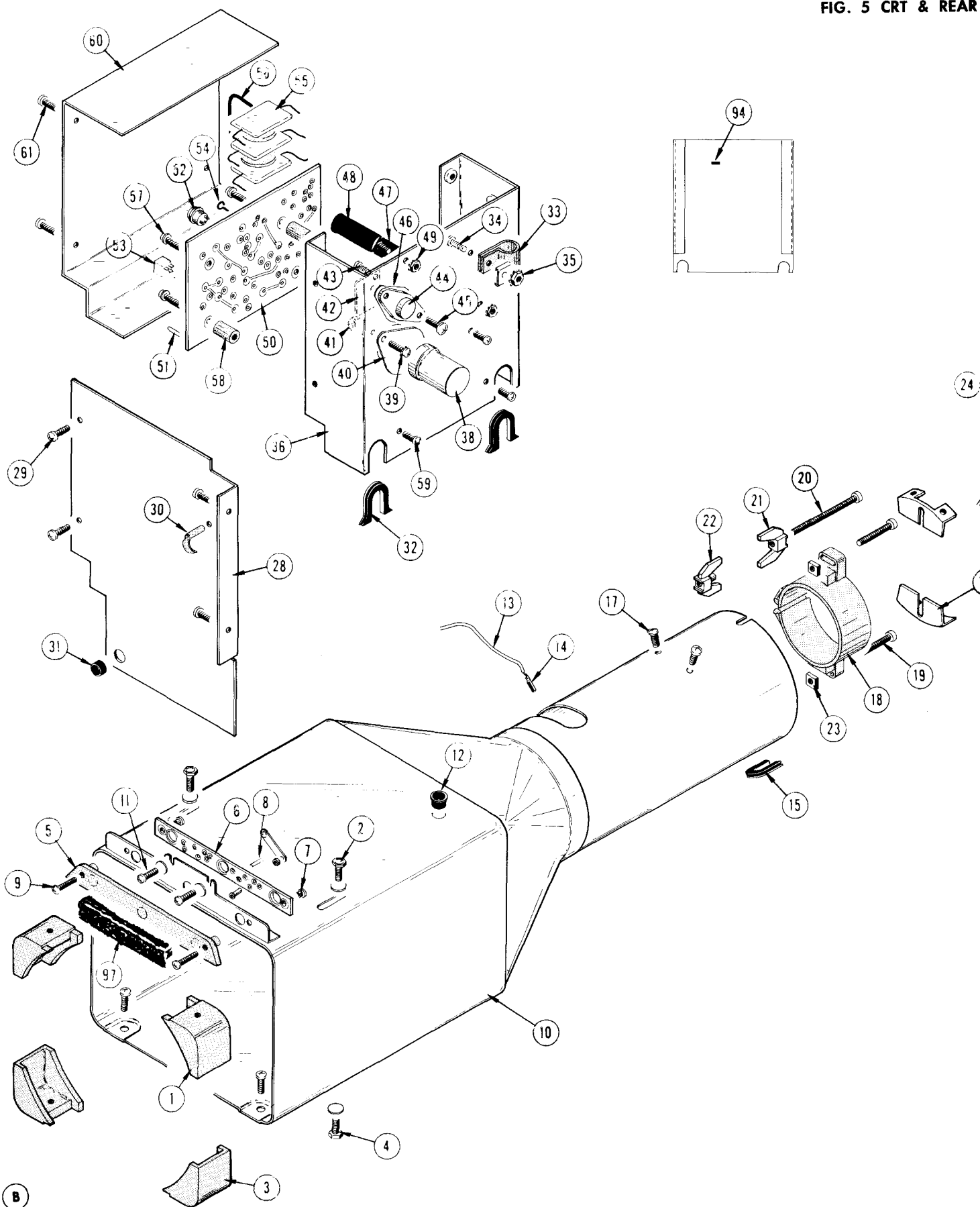
FIG. 5 CRT & REAR
